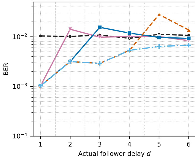
(b) BER vs. follower delay
