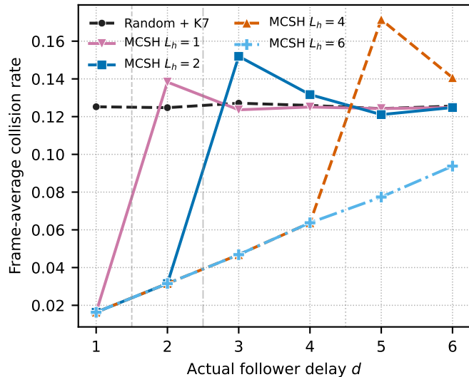
(a) Collision vs. follower delay (dashed lines = L_h boundaries)
