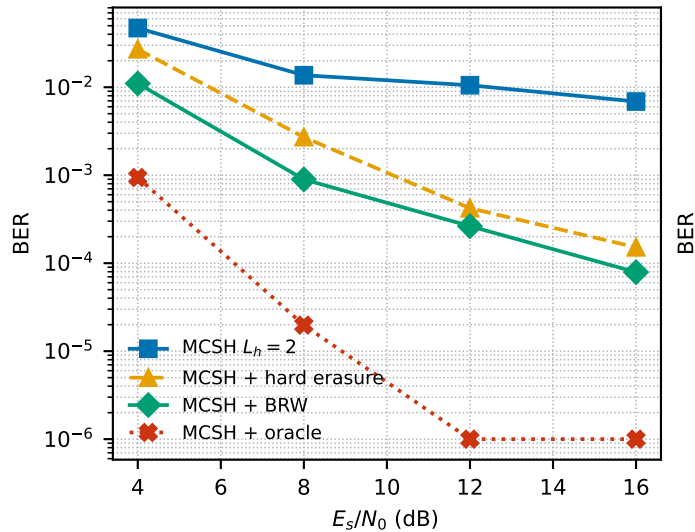
(a) Receiver ablation under sweep
