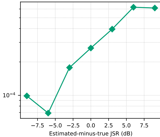
(b) BRW jammer-variance mismatch
