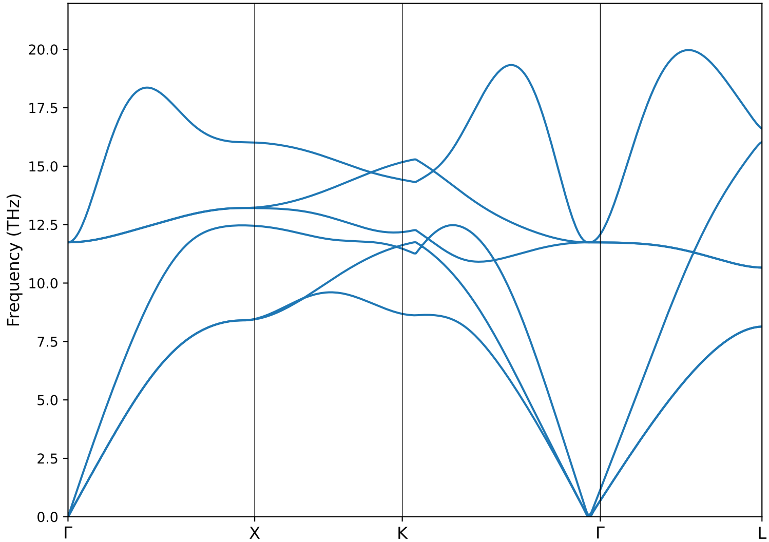
Phonon Dispersion
