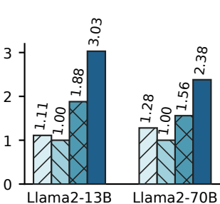
Norm. Throughput
