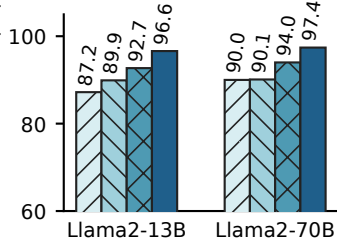
SLO Attainment (%)
