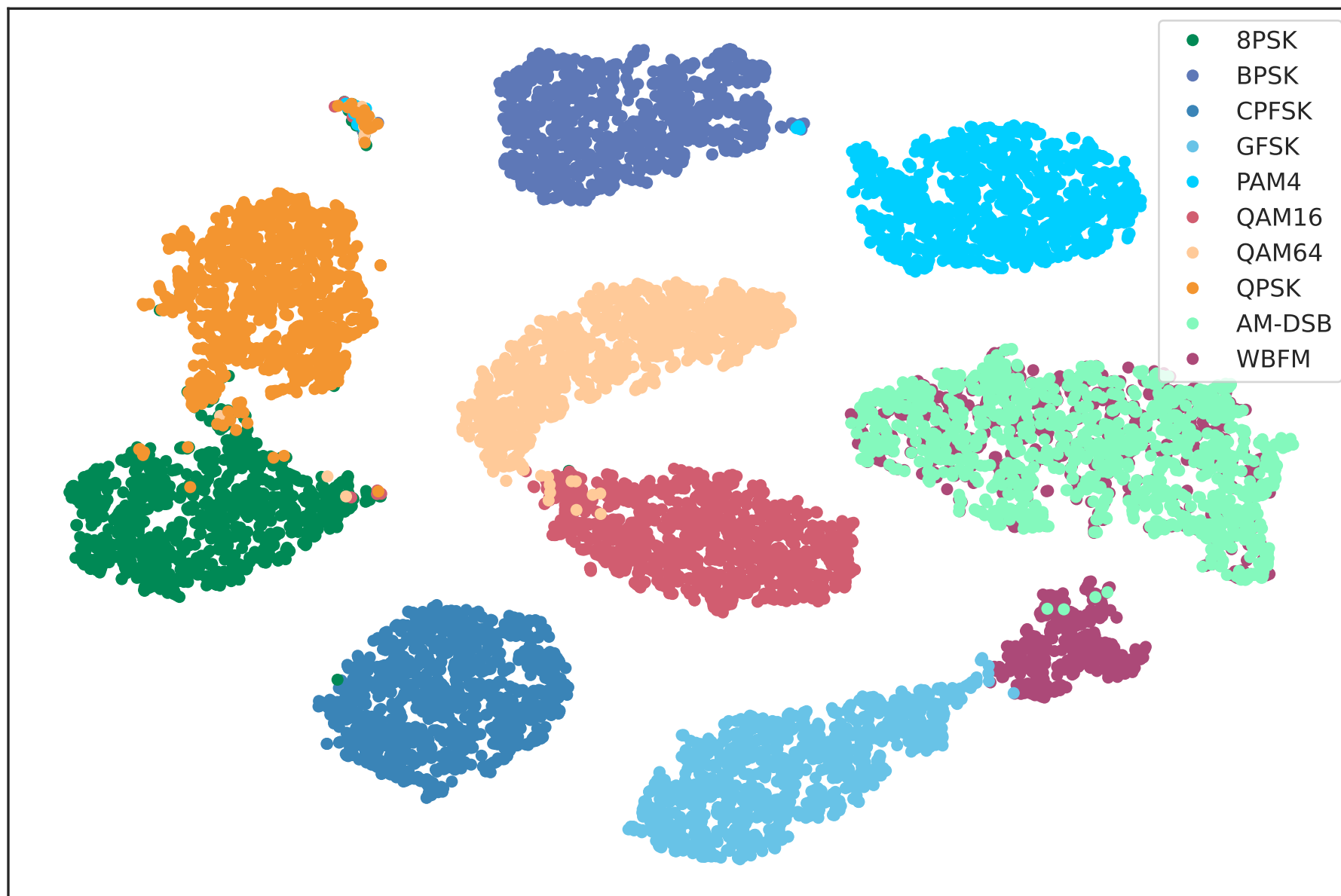
Visualization of t-SNE method at SNR = 0dB
