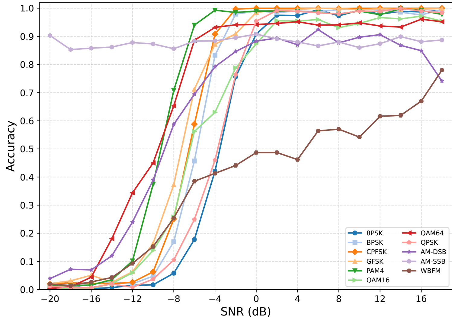
IQFormerLite on RadioML2016.10A
