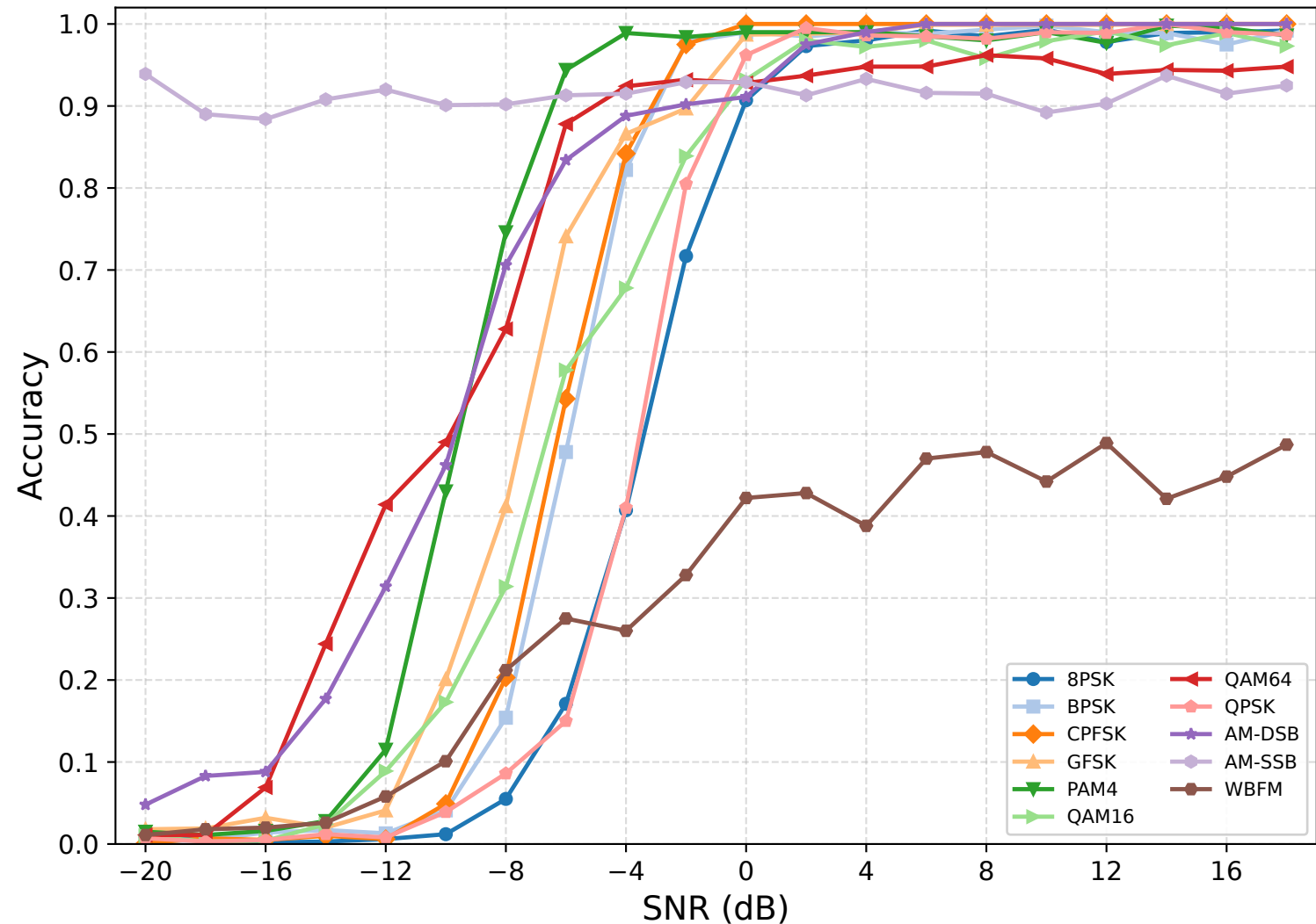
IQFormer on RadioML2016.10A
