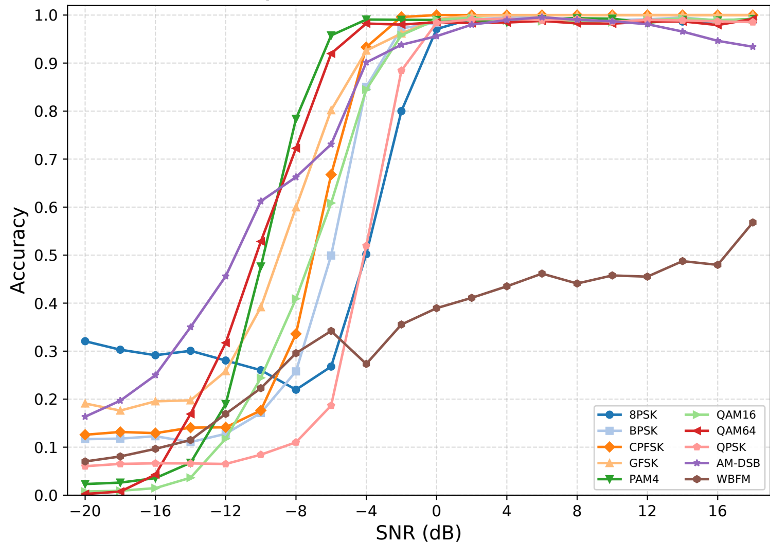
IQFormer on RadioML2016.10B
