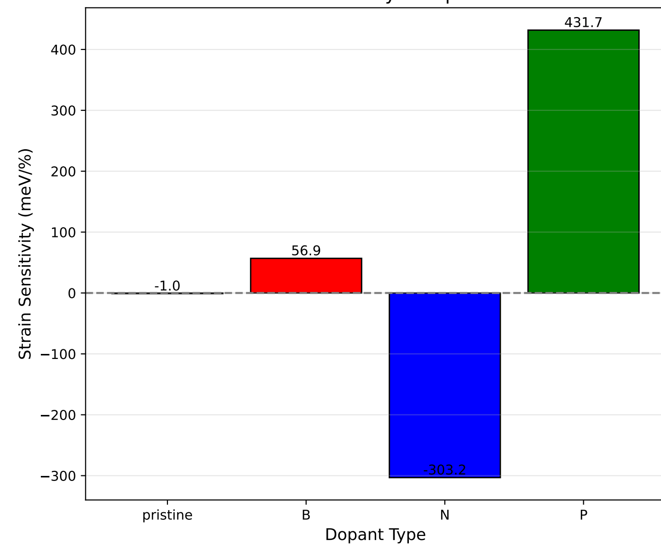
Strain Sensitivity Comparison
