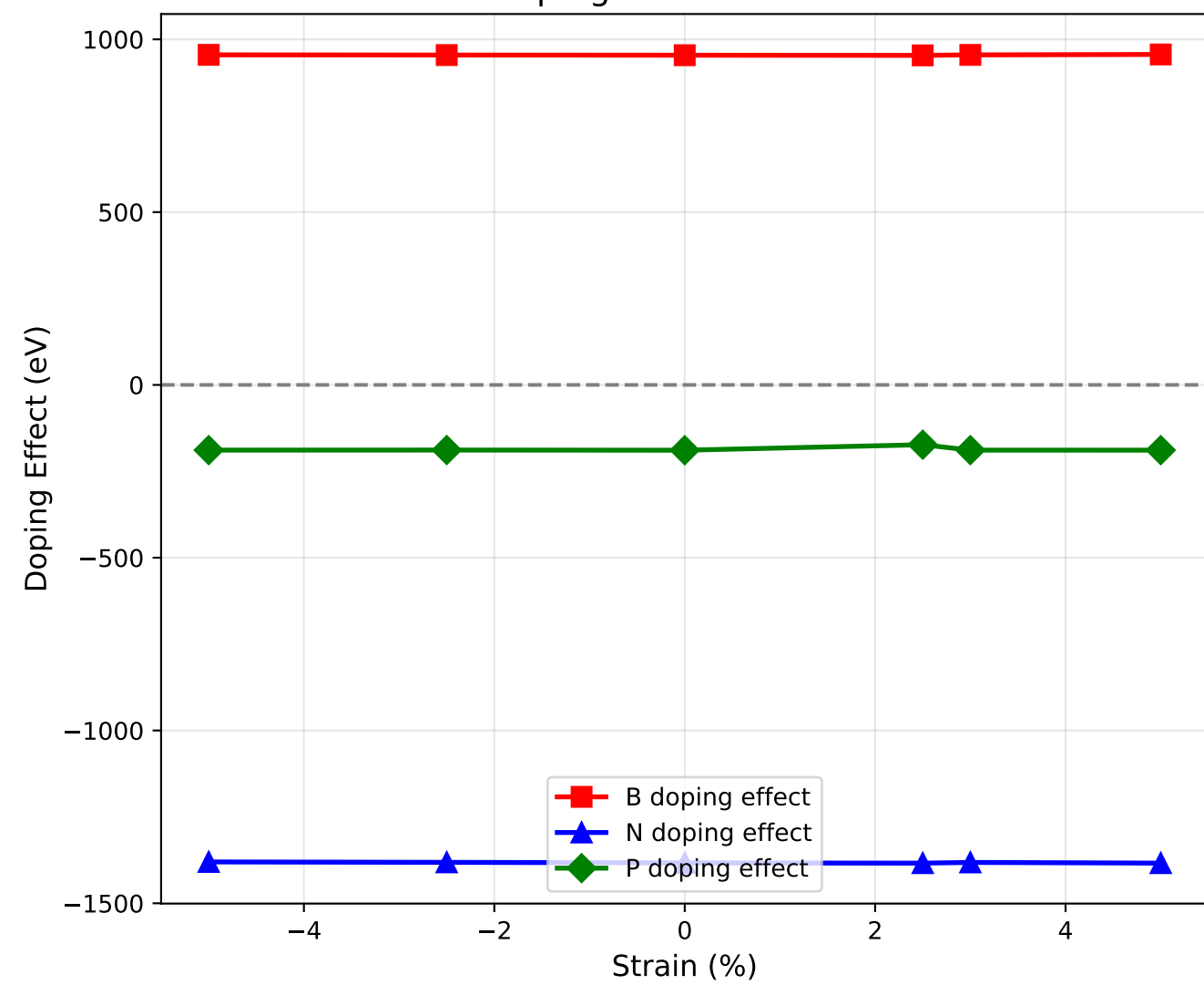
Doping Effect vs Strain
