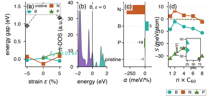
FIG. 1. Coupled (\epsilon, \delta) response in doped qHP C_{60} (PBE+D3). (a) HOMO–LUMO gap vs. strain. (b) \pi -DOS for B @ \epsilon=0 (Electron SI palette). (c) Mechanical \alpha . (d) S(n) at +3%; inset: Exp. 4 IPR/ J .
