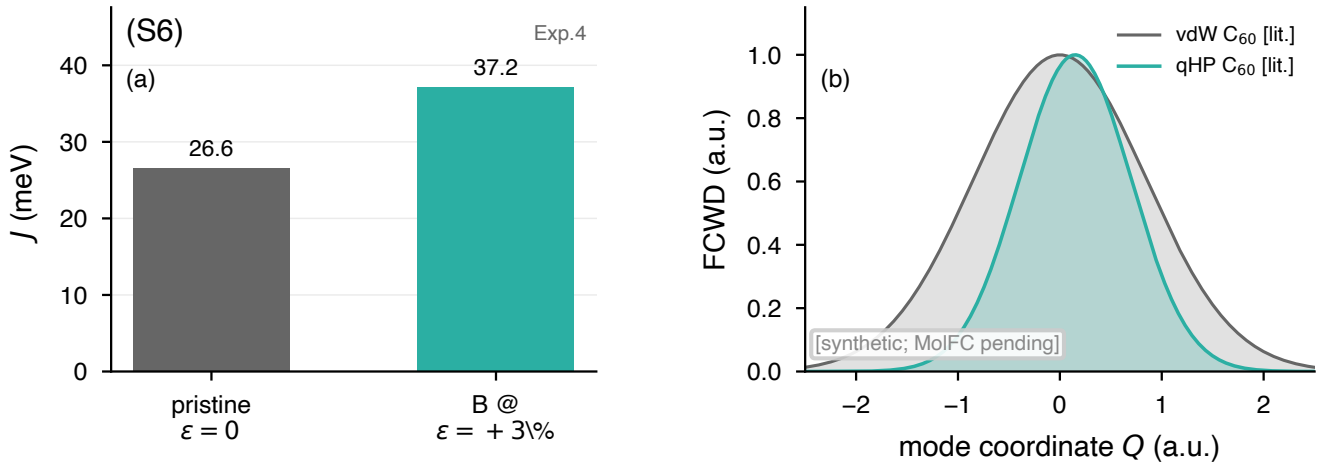
FIG. 3. Transport-adjacent observables: (a) nearest-neighbor J from Exp. 4 audit (PBE+D3, two verified tetramer points); (b) illustrative FCWD envelope (Electron SI MolFC/GF methodology [synthetic placeholder; tetramer MolFC pending]).
