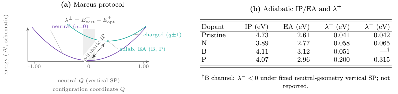
FIG. 1. Marcus reorganization energies from charged-state geometry optimizations and vertical single-points at the neutral geometry. Panel (a) schematically defines the vertical–adiabatic decomposition following Ref. 1; panel (b) tabulates adiabatic IP/EA and \lambda^{\pm} = E_{\text{vert}}^{\pm} - E_{\text{opt}}^{\pm} for pristine and B/N/P tetramers. The electron-channel \lambda^{-} for B is unphysical under the fixed neutral-geometry vertical protocol and is excluded (Limitations).
