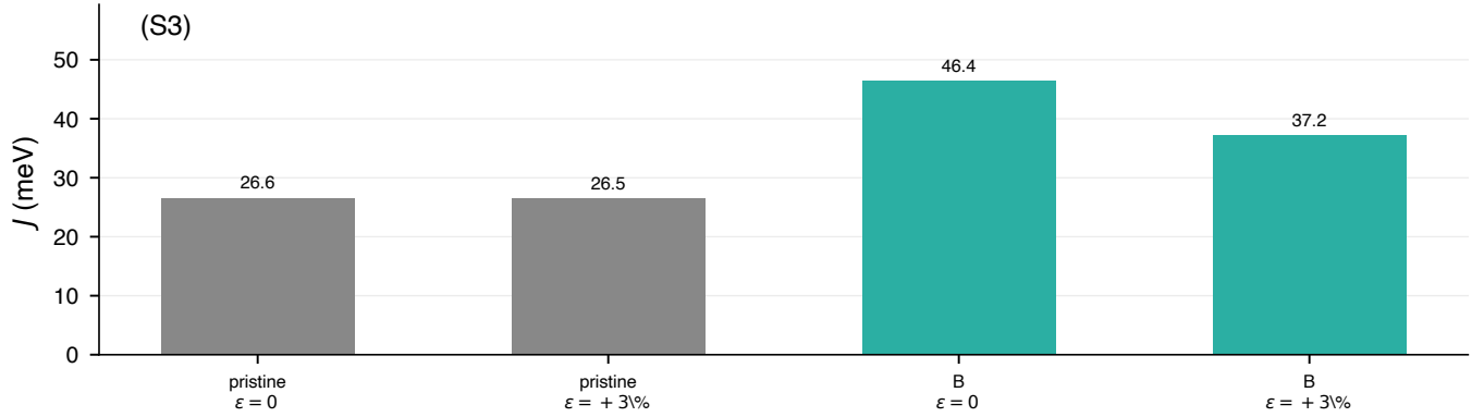
FIG. 2. Nearest-neighbor electronic coupling J on the tetramer dimer grid (pristine and B-doped cells at \epsilon=0 and +3\% ; PBE+D3). Companion inverse-participation-ratio values for the same four corners are tabulated in the open data release (Methods).
