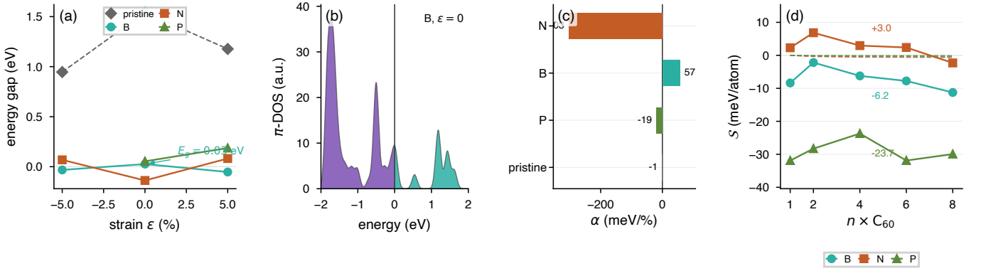
FIG. 1. Coupled (\epsilon, \delta) response in doped qHP C_{60} (PBE+D3). (a) HOMO-LUMO gap vs. strain. (b) \pi -DOS for B @ \epsilon=0 (color scheme follows Ref. 3). (c) Mechanical \alpha . (d) S(n) at +3%; n=4 values annotated; IPR/ J in Supplemental Material Fig. S6.
