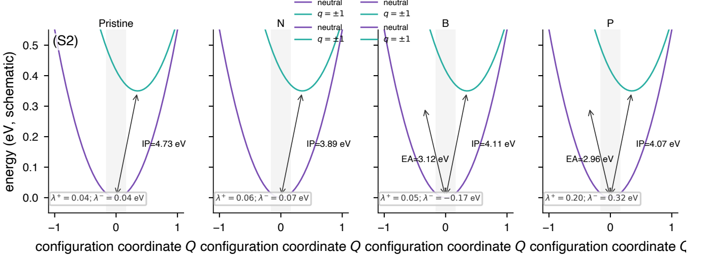
FIG. 3. Marcus reorganization energies (12/12 charged-state geometry optimizations; eight vertical single-points at the neutral geometry). Pristine \lambda^\pm = 0.041/0.042 eV; N \lambda^+ = 0.058/\lambda^- = 0.065 eV; B \lambda^+ = 0.051 eV; P \lambda^+ = 0.200/\lambda^- = 0.315 eV. The electron-channel reorganization energy \lambda^- for B doping is unphysical under the fixed neutral-geometry vertical protocol and is excluded (Limitations).
