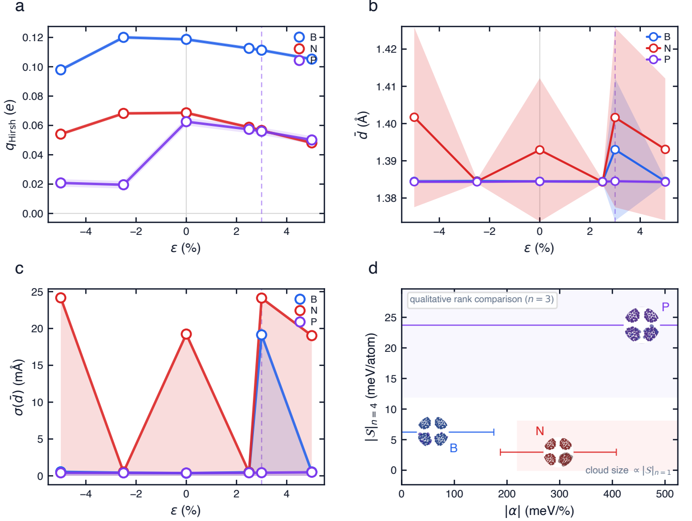
FIG. 3. Microscopic strain paths and \alpha - |\mathcal{S}| rank comparison ( n=3 dopants). (a) Hirshfeld q(\epsilon) for B/N/P (six-point paths; dotted guide at +3\% ). (b) Nearest-neighbor \bar{d}(\epsilon) with \pm\sigma bands. (c) Local disorder path \sigma(\bar{d})(\epsilon) . (d) Reference-map |\alpha| vs. periodic |\mathcal{S}|_{n=4} (marker area \propto |\mathcal{S}|_{n=1} ; horizontal bars: linear-fit standard errors on the six-point strain grid). N inverts a naive |\alpha| \rightarrow |\mathcal{S}| expectation; with only three dopants this panel reports qualitative ranking, not Pearson, R^2 , or Spearman statistics.
