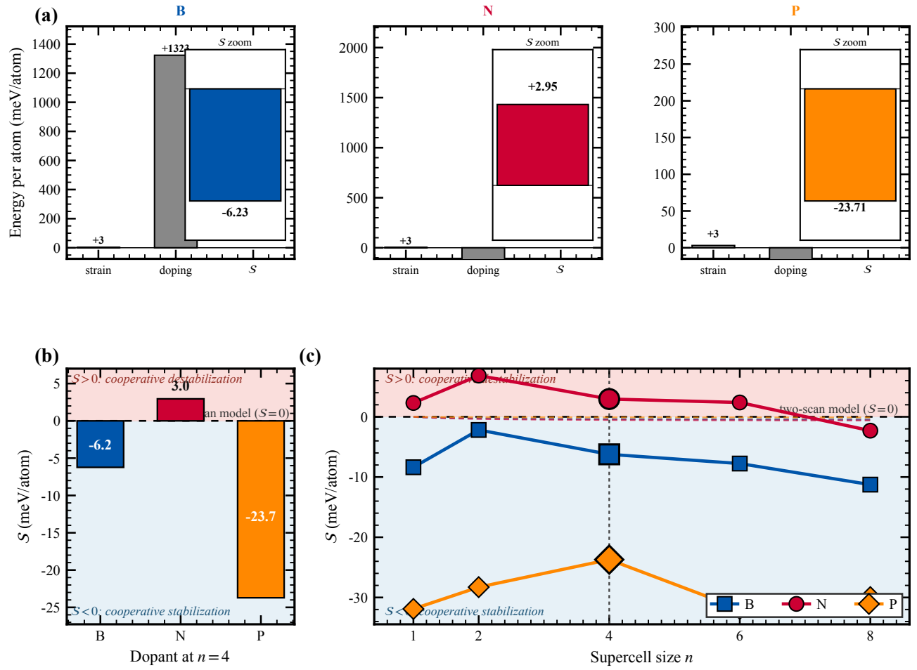
FIG. 3. Non-additive energy decomposition (Exp. 10, \epsilon = +3\% ). (a) Per-atom contributions: \Delta E_{\text{strain}} , \Delta E_{\text{dop}} , and cross term S at n = 4 (bars from sdc_exp10_results.json ). (b) S by dopant at tetramer scale; blue/red bands: cooperative stabilization/destabilization. (c) S(n) persistence to n = 8 .
