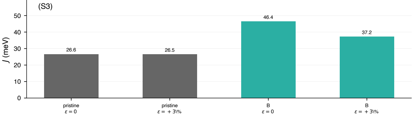
FIG. 4. Nearest-neighbor electronic coupling J on the tetramer dimer grid (pristine and B-doped cells at \epsilon=0 and +3\% ; PBE+D3). Companion inverse-participation-ratio values for the same four corners are tabulated in the open data release (Methods).
