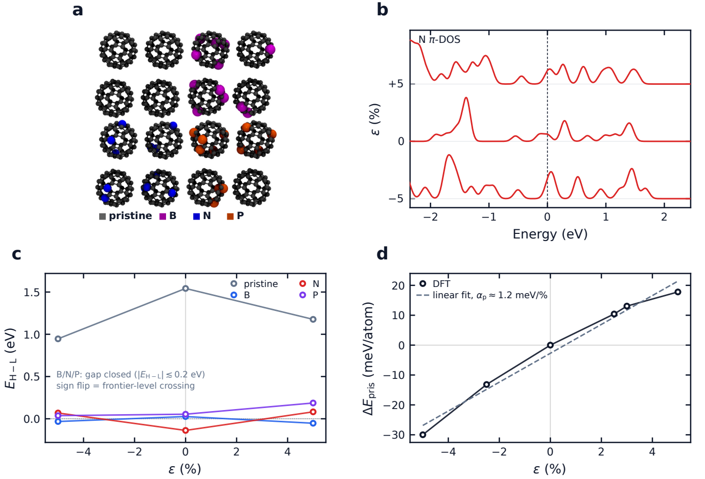
FIG. 1. Archived tetramer cluster map (PBE+D3). Cartesian coordinates are not affinely scaled; labeled \epsilon points change only the vacuum box. (a) qHP C_{60} tetramers at the archived \epsilon=0 snapshot: pristine (top left), B (top right), N (bottom left), P (bottom right), with substituent sites highlighted (covalent-radius excess in Table V). Heteroatoms and the key below the mosaic use CPK colors, which differ from the trajectory palette of panels (c) and (d). (b) N \pi -DOS vs. energy, stacked by the archived vacuum-box label ( E_F=0 ). (c) Frontier HOMO-LUMO separation E_{H-L} from the archived \pi -DOS spectra. Pristine keeps a 1.0–1.5 eV gap; all three substituted cages close it to |E_{H-L}| \lesssim 0.2 eV, and the residual separation changes sign because the frontier levels cross—a gap-closure indicator, not a negative gap. PBE underestimates gaps, so only the pristine-vs.-substituted contrast is interpreted. These spectra are not monolayer biaxial-strain paths. (d) Pristine cluster-map \Delta E vs. vacuum-box label (not a monolayer mechanical \alpha ). Periodic joint-load four-corner audits are in Fig. 2.
