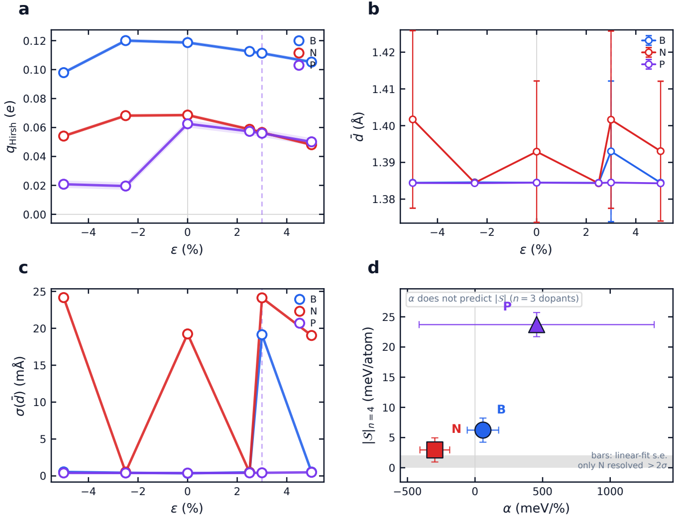
FIG. 3. Charge vs. geometry diagnostics and a qualitative rank comparison ( n=3 dopants). (a) Periodic Hirshfeld q(\epsilon) for B/N/P on affinely strained n=1 cells (six-point paths; dotted guide at +3\% ). This panel is a valid strain-path charge diagnostic. (b) Nearest-neighbor \bar{d} vs. vacuum-box label from archived tetramer XYZ (not an affine monolayer strain path). (c) Local disorder \sigma(\bar{d}) on the same frozen cluster map. (d) Cluster-map |\alpha| vs. periodic |S|_{n=4} (marker area \propto |S|_{n=1} ; horizontal bars: linear-fit standard errors on the six-point cluster map). The cluster |\alpha| is a configuration diagnostic, not a monolayer strain coefficient. N inverts a naive |\alpha| \rightarrow |S| expectation; with only three dopants this panel reports qualitative ranking, not Pearson, R^2 , or Spearman statistics.
