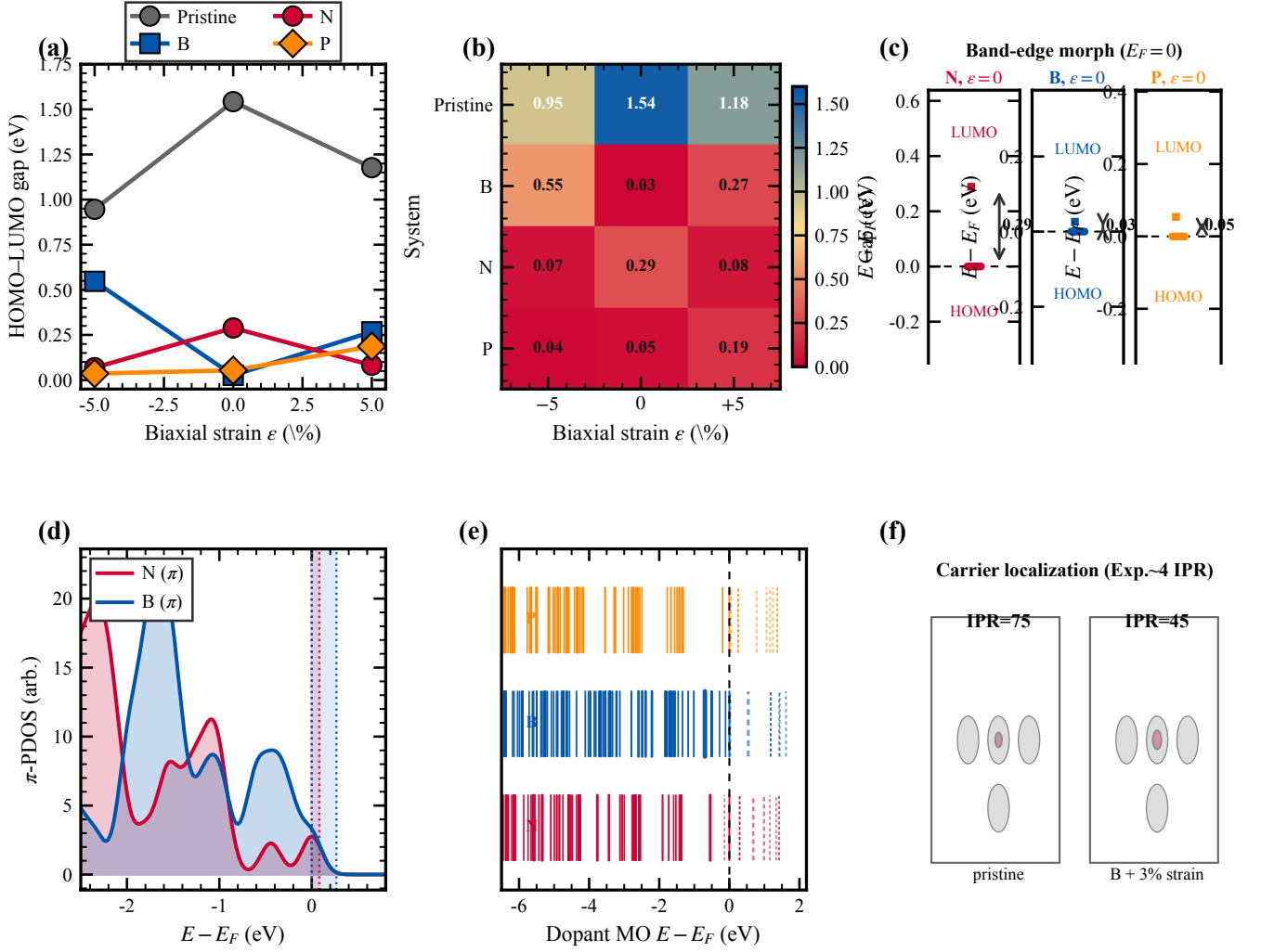
FIG. 2. Electronic morphology (Exp. 7, Exp. 4). (a) Gap vs. strain. (b) Gap heatmap. (c) Band edges at \epsilon = 0 . (d) \pi -PDOS at +5%. (e) Dopant MO spectrum. (f) IPR localization schematic.
