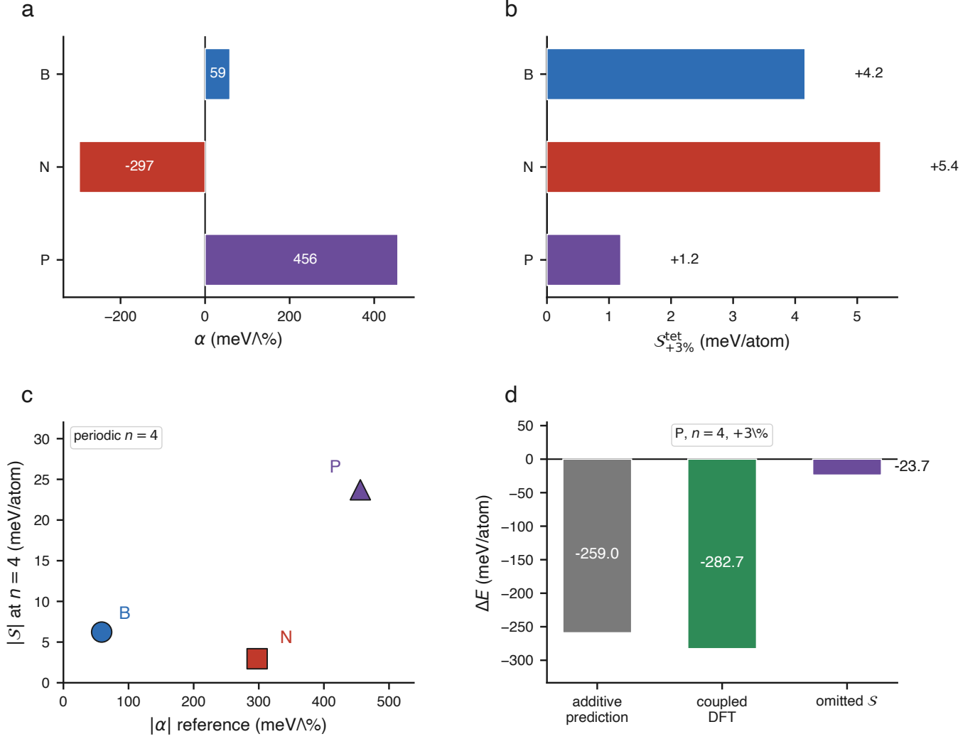
FIG. 3. \alpha - S decoupling and additive-model error. (a) Reference-placement tetramer \alpha (PBE+D3 rigid; same site map as the periodic S audit). (b) Matched-functional tetramer S^{\text{tet}}_{+3\%} on the same map. (c) Correlation of reference |\alpha| with periodic |S| at n=4 : N has large |\alpha| but small |S| (decoupling). (d) Additive vs. coupled energy shifts for P at n=4 , +3%: sequential screening misses S = -23.7 meV/atom.
