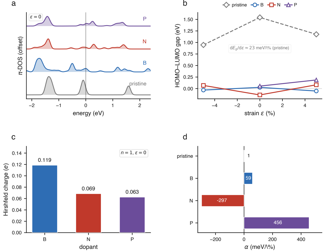
FIG. 1. Electronic structure and intrinsic strain response of pristine and B/N/P-doped qHP C 60 (PBE+D3 unless noted). (a) Offset \pi -DOS at \epsilon=0 (Fermi level at 0 eV). (b) HOMO-LUMO gap vs. biaxial strain (tetramer electronic archive; PBE). (c) Hirshfeld charge on the dopant at n=1, \epsilon=0 . (d) Linear strain coefficient \alpha on the reference placement map (rigid PBE+D3).
