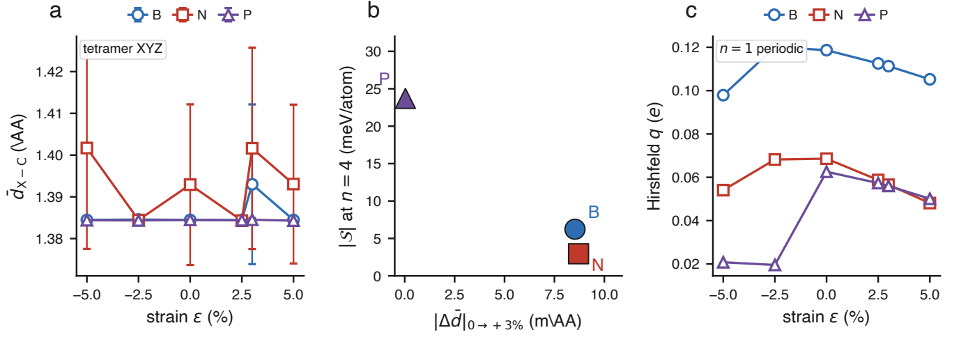
FIG. 4. DFT local geometry and population under biaxial strain. (a) Mean dopant-C nearest-neighbor distance \bar{d}_{X-C}(\epsilon) from tetramer XYZ (error bars: site standard deviation). P remains flat across the strain grid; B and N show larger local response at selected strains. (b) Strain-induced stretch |\Delta \bar{d}| ( 0 \rightarrow +3\% ) vs. periodic |S| at n=4 : P has vanishing \Delta \bar{d} yet the largest cross term. (c) Hirshfeld charge q(\epsilon) on the dopant site ( n=1 periodic). N shows the largest fractional charge swing while carrying the smallest |S| at n=4 . Panels (a)–(c) are DFT observables; mismatch thresholds for design rules remain in Table II.
