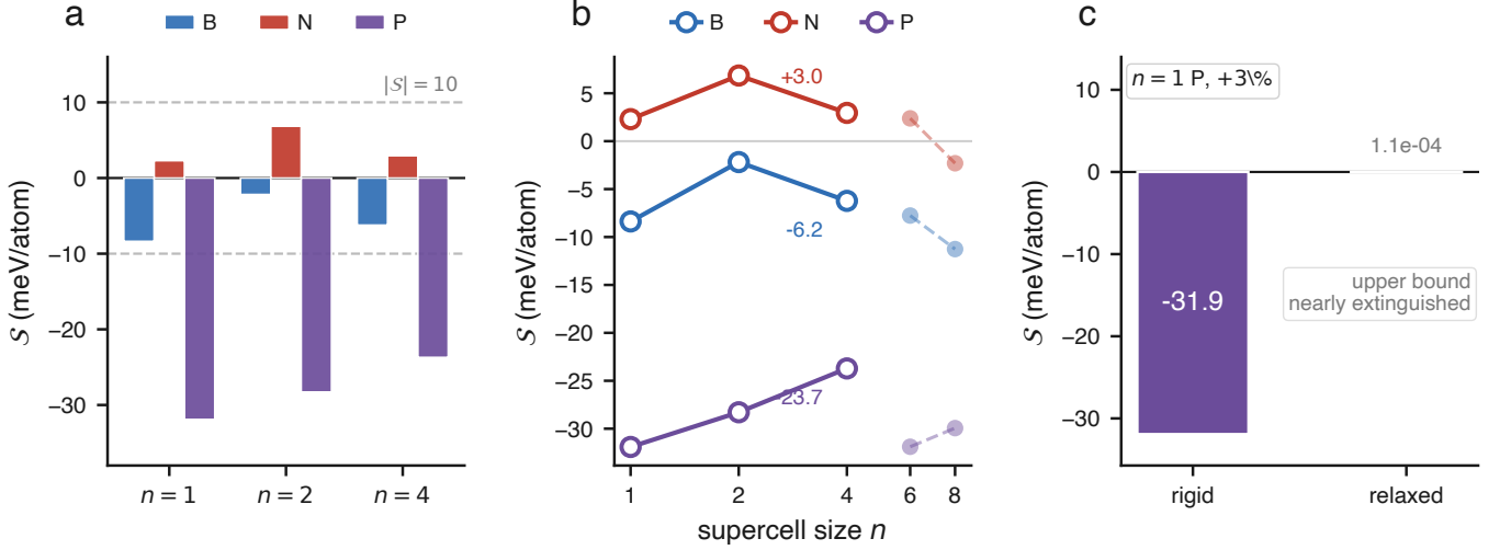
FIG. 2. Non-additive synergy order parameter S under +3% biaxial strain (PBE+D3 rigid protocol unless noted). (a) Grouped S for n=1, 2, 4 (Table III); dashed lines mark |S|=10 meV/atom; peak |S|=31.9 meV/atom for P at n=1 . (b) S(n) size evolution (solid: matched 400 Ry core n \leq 4 ; dashed: 350 Ry n \geq 6 ). (c) Rigid vs. ionically relaxed S for periodic n=1 P at +3%: the rigid value is an upper bound that is nearly extinguished upon relaxation.
