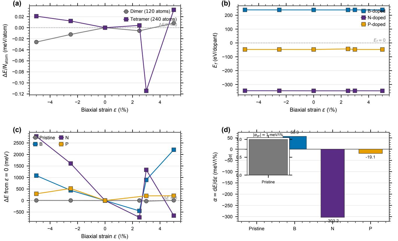
FIG. 1. Non-additive strain-doping coupling in graphullerene tetramers (Exp. 5, PBE+D3). (a) Pristine \Delta E/N_{\text{atom}} vs biaxial strain for dimer and tetramer (near-insensitive). (b) Substitution energy E_f vs strain for B/N/P dopants. (c) Total-energy change \Delta E from \epsilon = 0 . (d) Strain sensitivity \alpha with inset highlighting |\alpha_{\text{pristine}}| \approx 1 \text{ meV}/\% vs |\alpha_N| \approx 303 \text{ meV}/\% .
