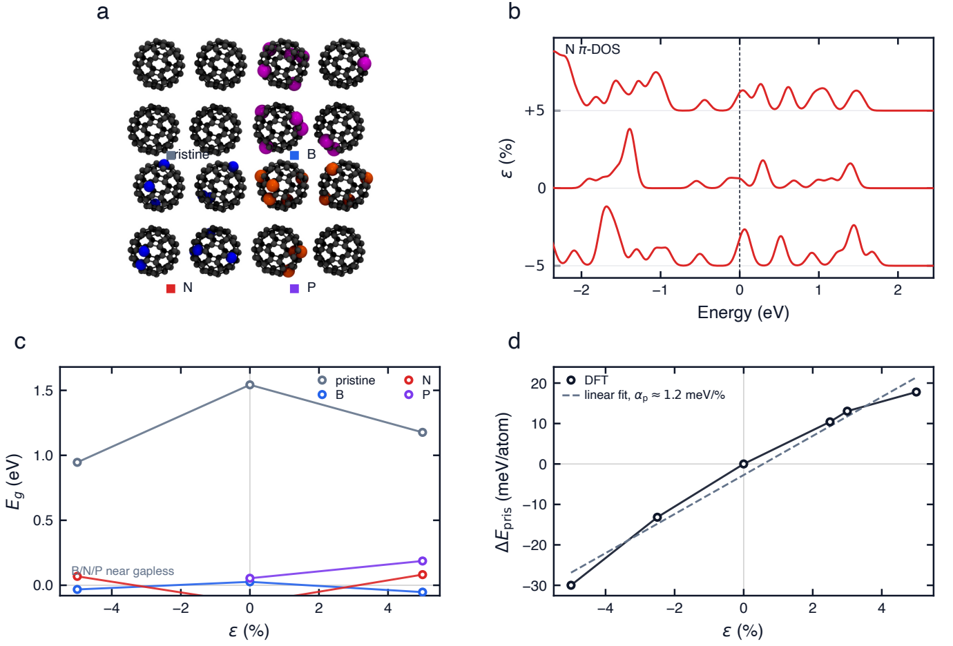
FIG. 1. Reference tetramer and one-parameter strain slices (PBE+D3). (a) qHP C 60 cages at \epsilon=0 . Heteroatoms are CPK; B/N/P labels follow the manuscript palette of (c) (Table V). (b) N \pi -DOS vs. energy, stacked by biaxial strain E_F=0 . (c) Gap E_g(\epsilon) ; B/N/P remain near gapless on this scale. (d) Pristine mechanical \Delta E(\epsilon) and linear \alpha . Joint-load four-corner audits are in Fig. 2.
