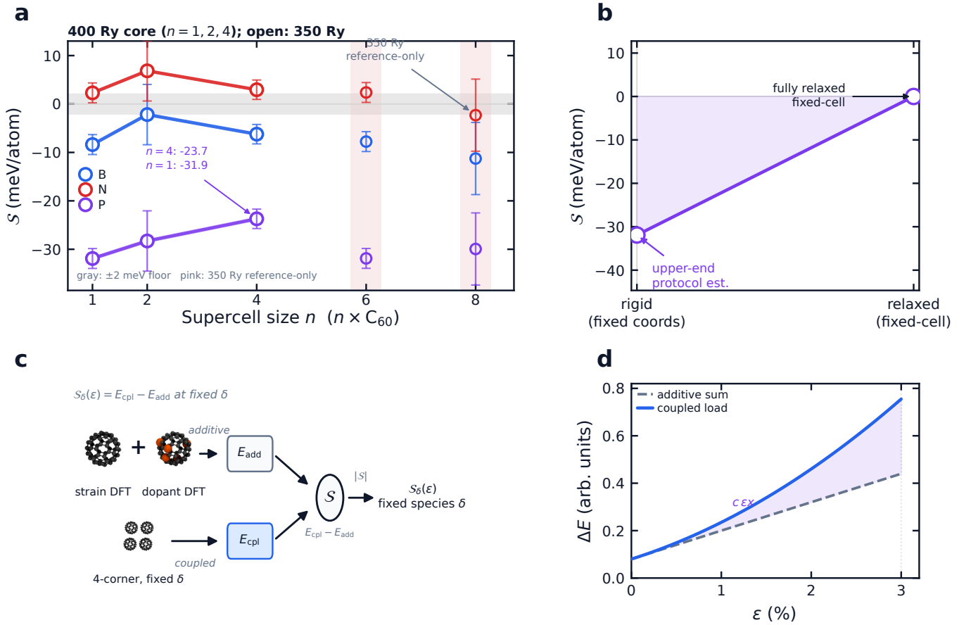
FIG. 2. Additive strain-dopant screening fails under constrained load. (a) Periodic +3% S(n, \delta) (gray band: \pm 2 meV/atom protocol resolution floor, not a statistical confidence interval). Filled markers and connecting lines are the matched 400 Ry core ( n=1, 2, 4 ). Open markers are n=6, 8 at 350 Ry, shown as reference only and not used for mechanistic or asymptotic inference. Error bars add the systematic offset of the pristine strain reference; the larger n=2 bar is that offset on the 400 Ry core, not a cutoff-tier marker (Table I). Pink columns mark only the 350 Ry sizes. On the matched core, headline n=4 P is -23.7 meV/atom and the span end n=1 is -31.9 meV/atom, while several B/N points sit near the floor, so the audit resolves a stratification and not a uniform failure of additivity. (b) Constrained fixed-coordinate diagnostic: an upper-end protocol estimate relative to the fully relaxed fixed-cell protocol studied here, not a universal bound on every constraint and not a second size-scaling panel. Periodic n=1 P at +3%: ionic relaxation suppresses the cross term to the reporting floor. Table II is a distinct tetramer boundary condition (vacuum box; coordinates not affinely strained): +1.19 \rightarrow -2.28 meV/atom (sign reversal and larger magnitude). It is not a retention ratio for the periodic grid. (c) Definition: additive sum of strain-only and substitution-only increments vs. the coupled four-corner total; S_\delta(\epsilon) is that gap at fixed dopant species \delta [Eq. (3)]. (d) Schematic E(\epsilon) at fixed species: the bilinear c\epsilon x term, with x a local composition coordinate, bends the coupled path away from the additive sum (cartoon, not a DFT fit).
