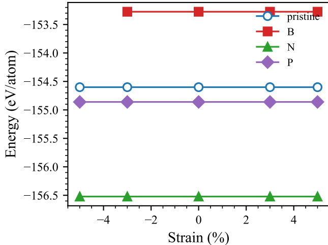
(b) Single C 60
