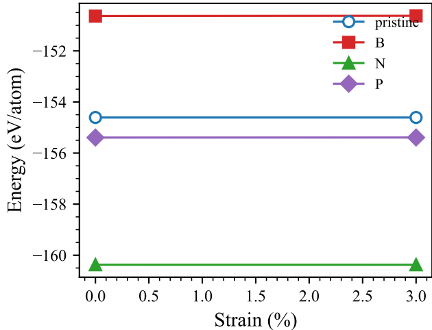
(a) C 60 dimer
