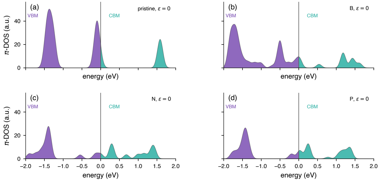
FIG. S1. \pi -projected density of states ( \pi -DOS) for pristine and B/N/P-doped tetramers at \epsilon=0 (PBE+D3). Valence band edges (purple) and conduction band edges (teal) follow the color scheme of Capobianco et al. [1]. Energy is relative to the Fermi level at 0 eV. Molecular-orbital isosurfaces are pending cube export.
