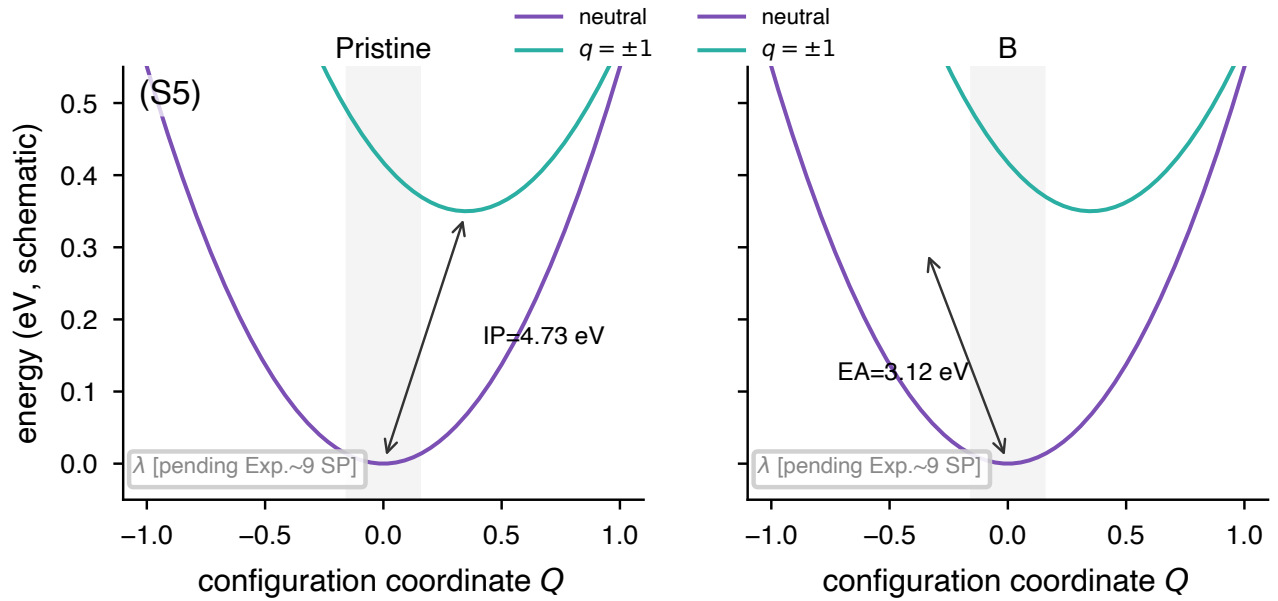
FIG. 2. Marcus configuration-coordinate schematic (Capobianco-style). Verified adiabatic IP/EA from converged Exp. 9 GEO-OPT pairs label the vertical arrows (pristine IP, B EA); \lambda panels remain [pending: vertical SP at neutral geometry]—see derived.lambda.eV in audit JSON.
