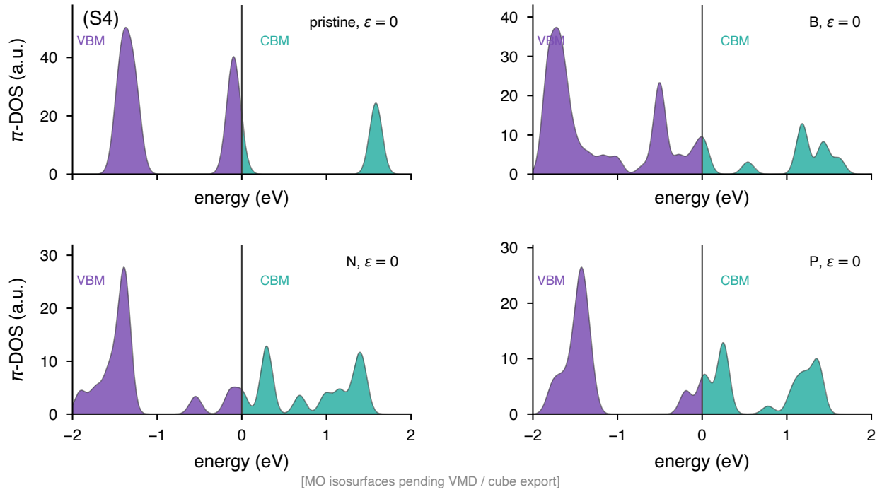
FIG. 1. \pi -projected DOS at \varepsilon=0 for pristine and B/N/P tetramers (Exp. 7 .pdos, PBE+D3). MO isosurfaces [pending: VMD + cube export]; band-edge labels follow E_F .
