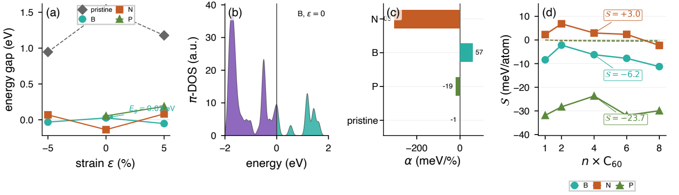
FIG. 1. Coupled (\epsilon, \delta) response in doped qHP C_{60} (PBE+D3). (a) HOMO-LUMO gap vs. strain. (b) \pi -DOS for B @ \epsilon=0 (color scheme follows Ref. 3). (c) Mechanical \alpha . (d) S(n) at +3%; n=4 values annotated; IPR/ J in Supplemental Material Fig. S6.
