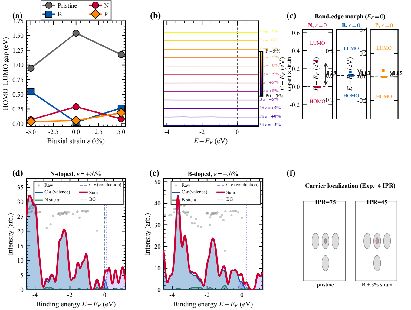
FIG. 2. Electronic morphology (Exp. 7, Exp. 4). (a) Gap vs. strain. (b) Stacked \pi -PDOS waterfall (dopant \times strain). (c) Band edges at \epsilon = 0 . (d-e) XPS-style PDOS deconvolution (N, B @ +5%). (f) IPR localization schematic.
