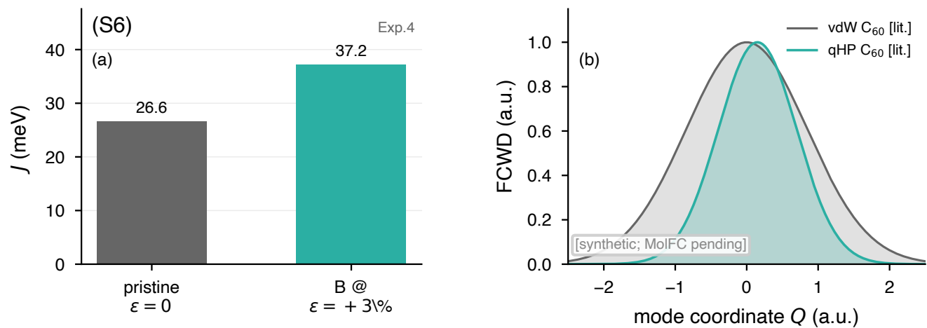
FIG. 3. Transport-adjacent observables: (a) nearest-neighbor J from Exp. 4 audit (PBE+D3, two verified tetramer points); (b) illustrative Franck-Condon weighted density (FCWD) envelope following Ref. 1 [ synthetic; MolFC replacement pending ].
