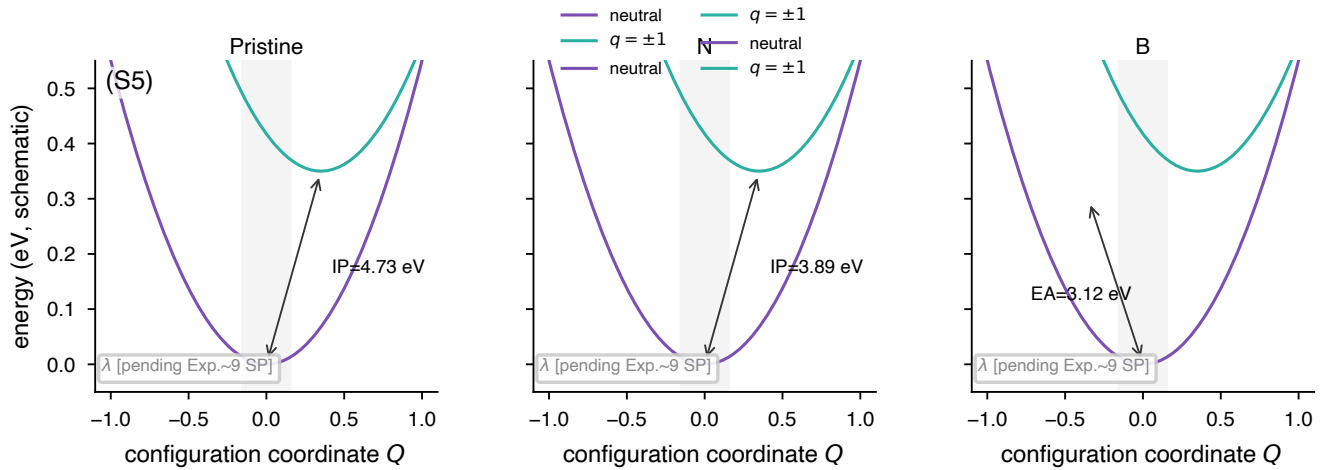
FIG. 2. Marcus configuration-coordinate schematic (Capobianco-style). Verified adiabatic IP/EA from converged Exp. 9 GEO-OPT pairs label the vertical arrows (pristine IP, N IP, B EA); \lambda panels remain [pending: vertical SP at neutral geometry]—see derived.lambda.eV in audit JSON.
