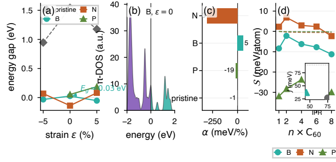
FIG. 1. Coupled (\epsilon, \delta) response in doped qHP C 60 (PBE+D3; Capobianco-style layout). (a) HOMO–LUMO gap vs. strain (Exp. 7; P @ -5\% excluded). (b) \pi -projected DOS for B @ \epsilon=0 [Exp. 7 .pdos; Electron SI valence purple / conduction teal]. (c) \alpha from Exp. 5 [table1_verification.json]. (d) S(n) at +3\% (15 points) [sdc_exp10_synergy_audit.json]; inset: Exp. 4 IPR/ J .
