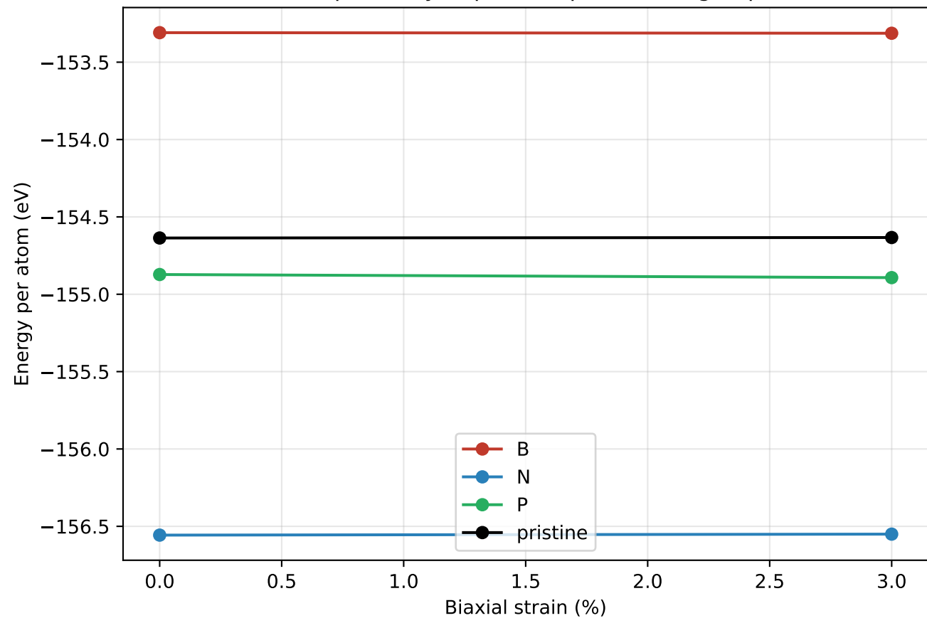
Strain response by dopant (Exp10 converged points)
