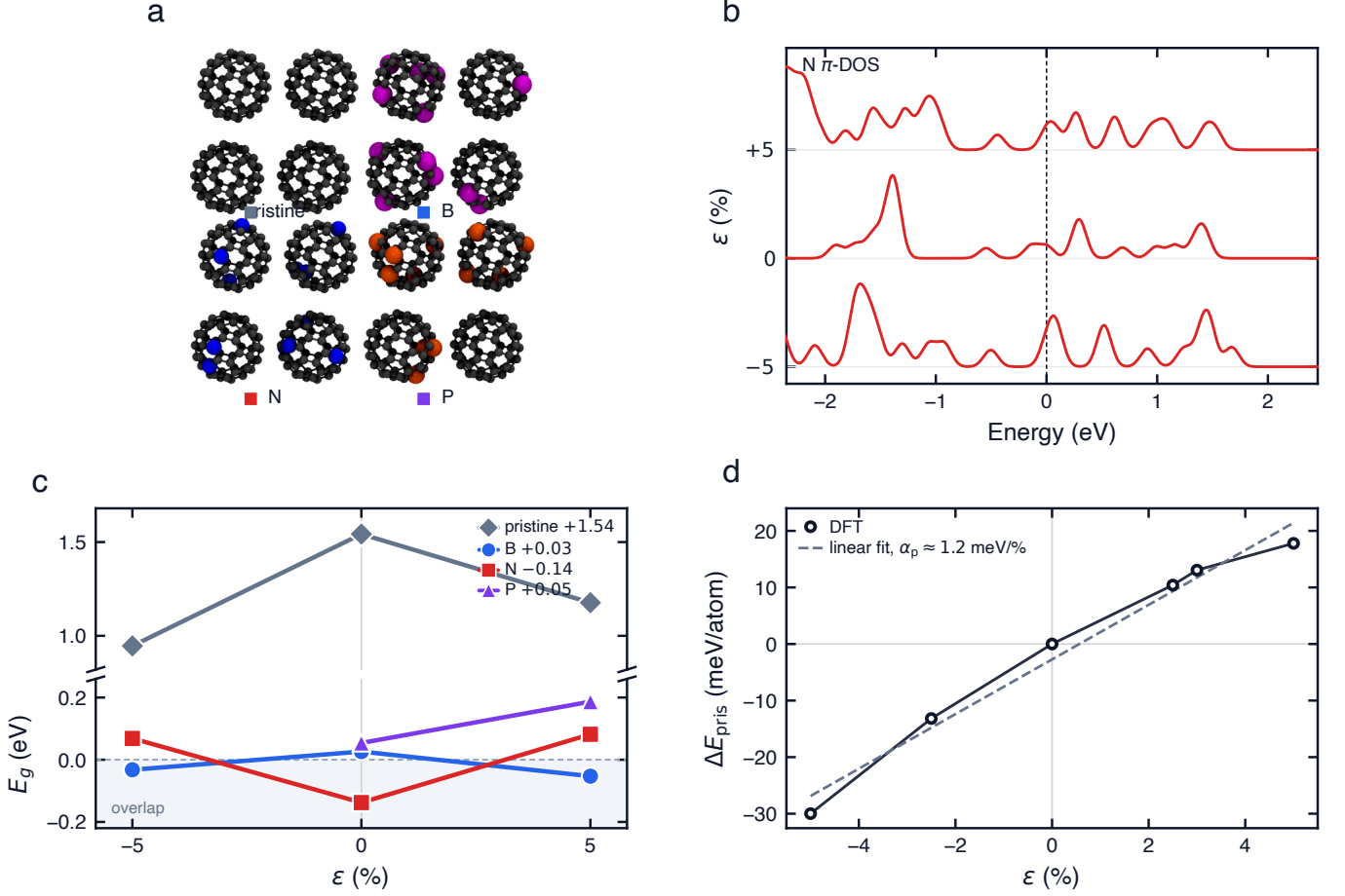
FIG. 1. Reference tetramer and one-parameter strain slices (PBE+D3). (a) qHP C_{60} cages at \epsilon=0 . Heteroatoms are CPK; B/N/P labels follow the manuscript palette of (c) (Table V). (b) N \pi -DOS vs. energy, stacked by biaxial strain E_F=0 . (c) Signed HOMO–LUMO gap E_g(\epsilon) on a broken axis (pristine open; B/N/P near gapless; E_g<0 is level overlap). Legend lists \epsilon=0 values. (d) Pristine mechanical \Delta E(\epsilon) and linear \alpha . Joint-load four-corner audits are in Fig. 2.
