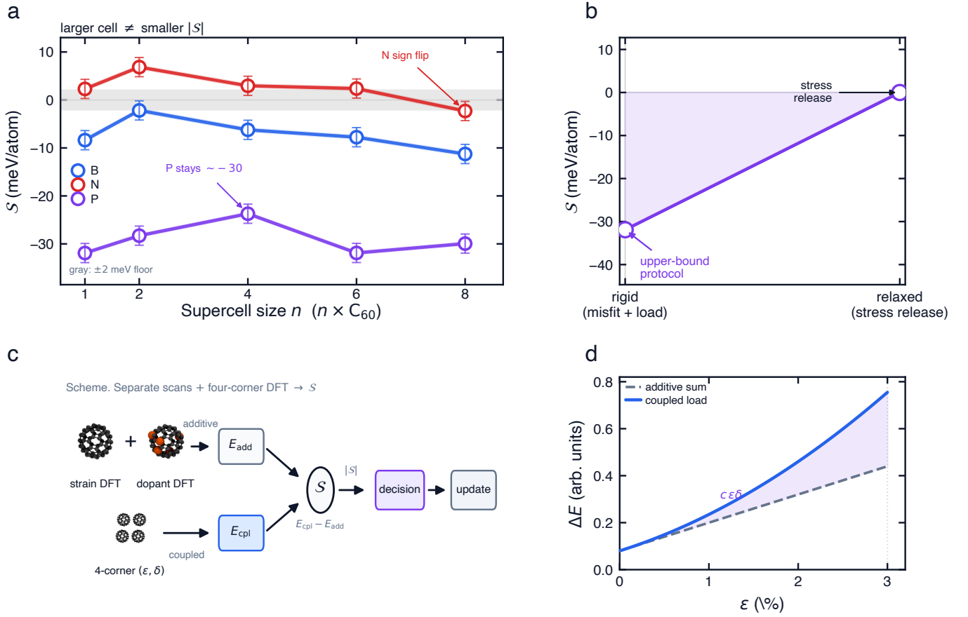
FIG. 2. Additive strain-dopant screening fails under constrained load. (a) Fifteen periodic +3% S(n, \delta) values vs. supercell size (markers: DFT; error bars and gray band: \pm 2 meV/atom protocol floor; Tables I and IV). |S| does not fall as 1/n : P remains \sim -24 to -32 meV/atom through n=8 ; N changes sign at n=8 . No S_\infty extrapolation. (b) Protocol bound, not a second size-scaling panel: periodic n=1 P at +3%, rigid vs. ionically relaxed S (near zero after stress release). The tetramer sign reversal in Table II is a different system. (c) Definition: additive sum of strain-only and substitution-only increments vs. the coupled four-corner total; S is that gap [Eq. (3)]. (d) Schematic E(\epsilon) at fixed composition: the bilinear c\epsilon\delta term bends the coupled path away from the additive sum (cartoon, not a DFT fit).
