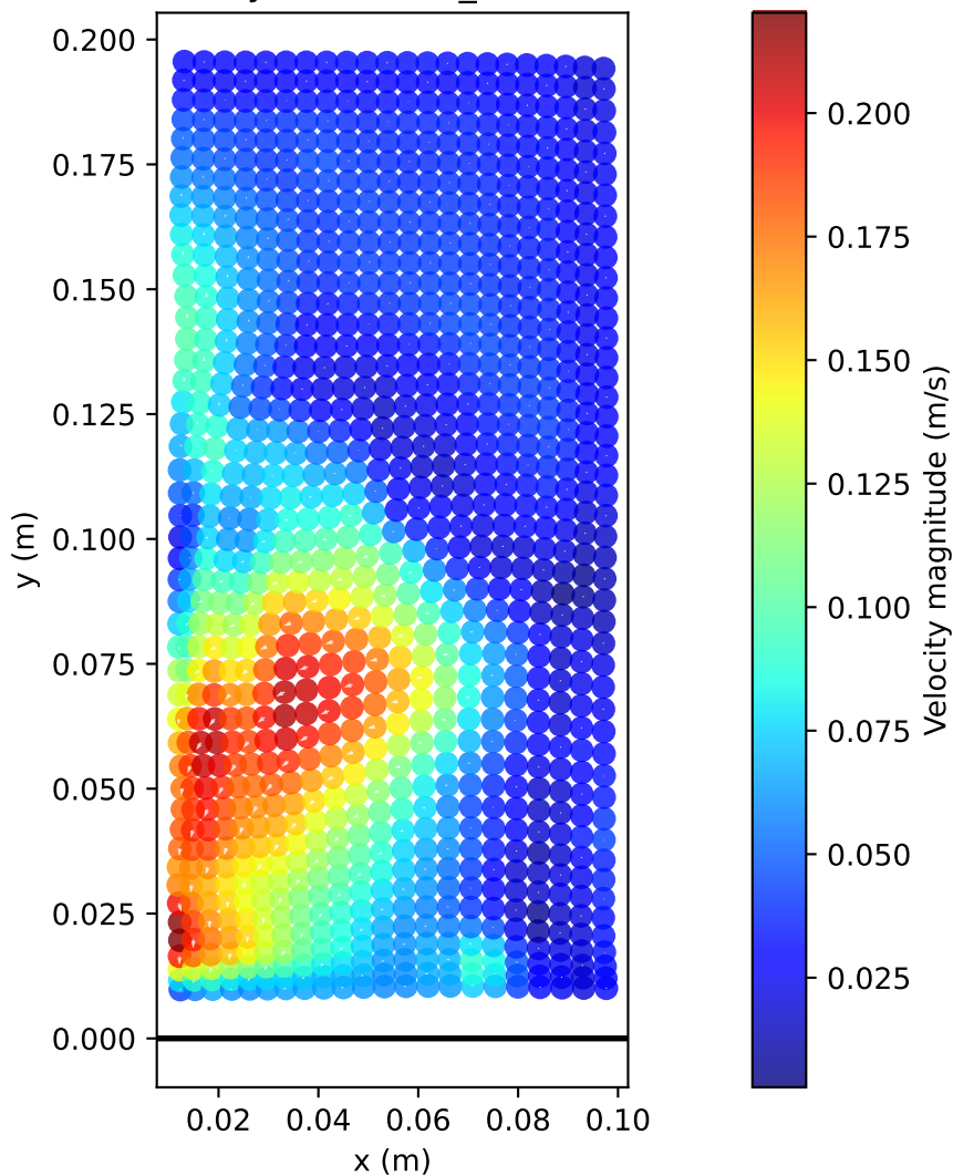
Velocity Field at t/t_{\text{ref}} = 1.00
