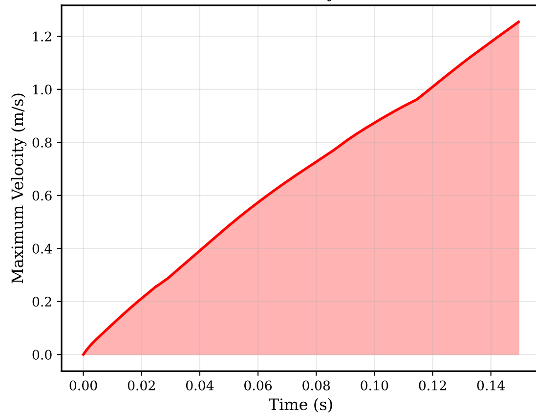
Wave Front Velocity
