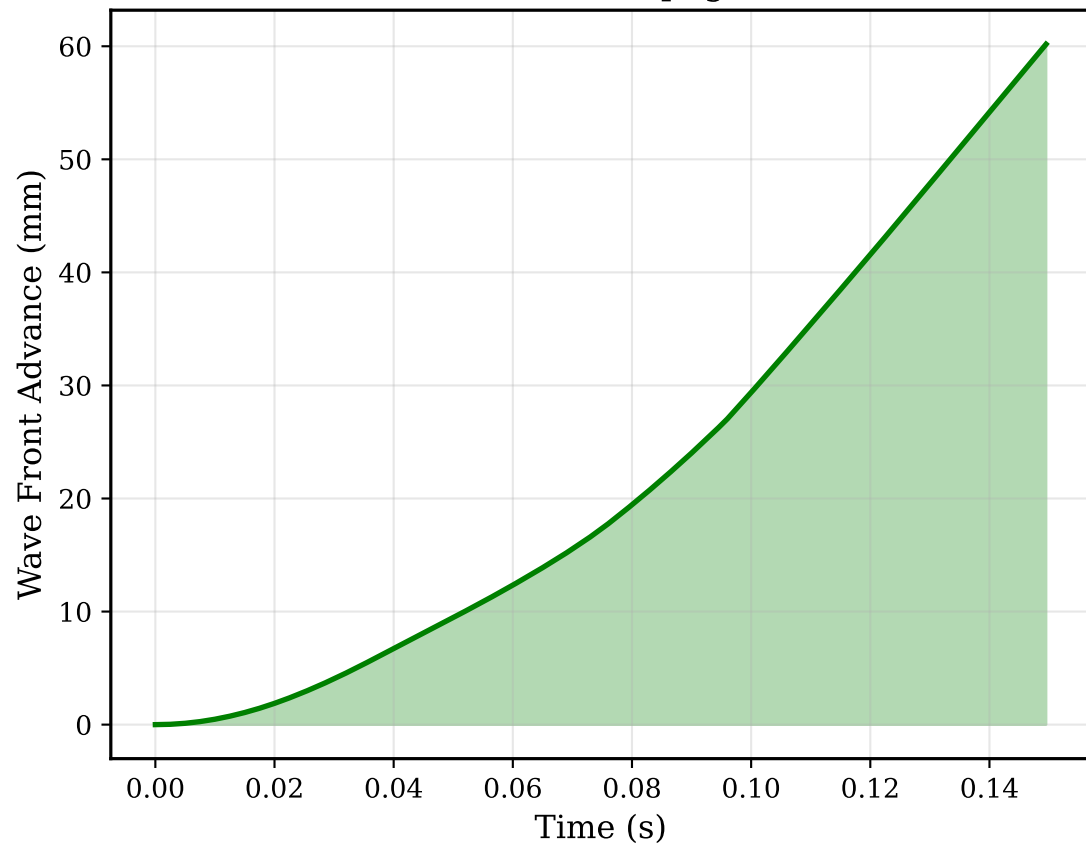
Wave Front Propagation
