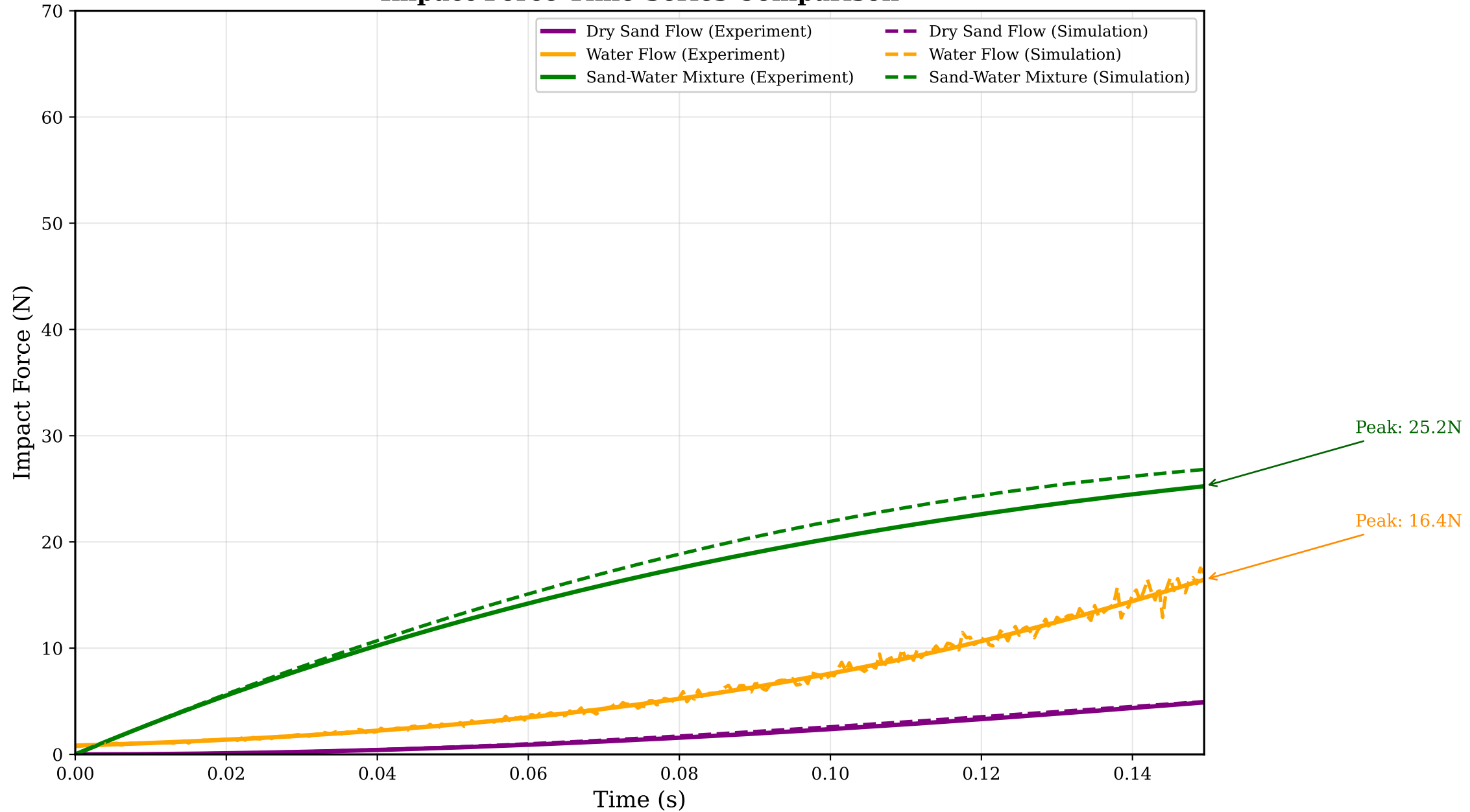
Impact Force Time Series Comparison
