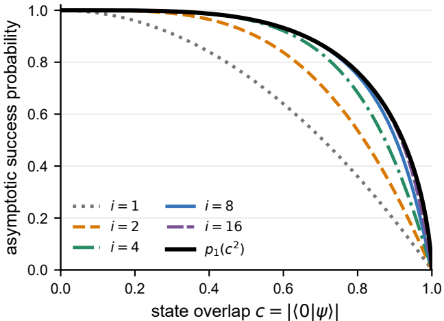
(a) P_\infty(i, c^2) \rightarrow p_1(c^2)
