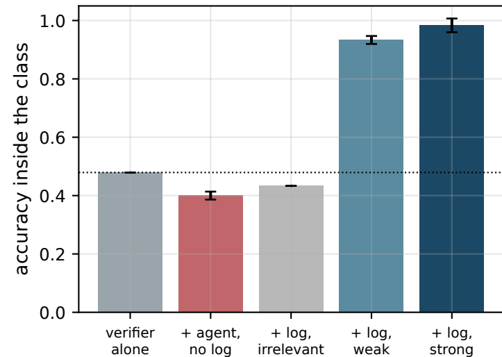
(a) accuracy by condition
