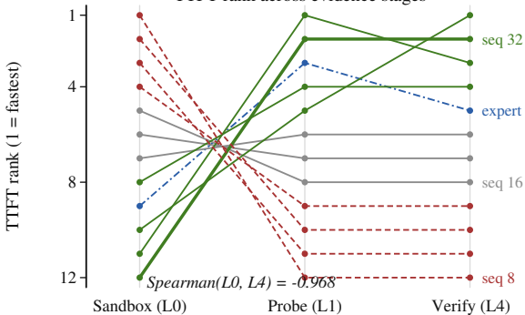
TTFT rank across evidence stages
