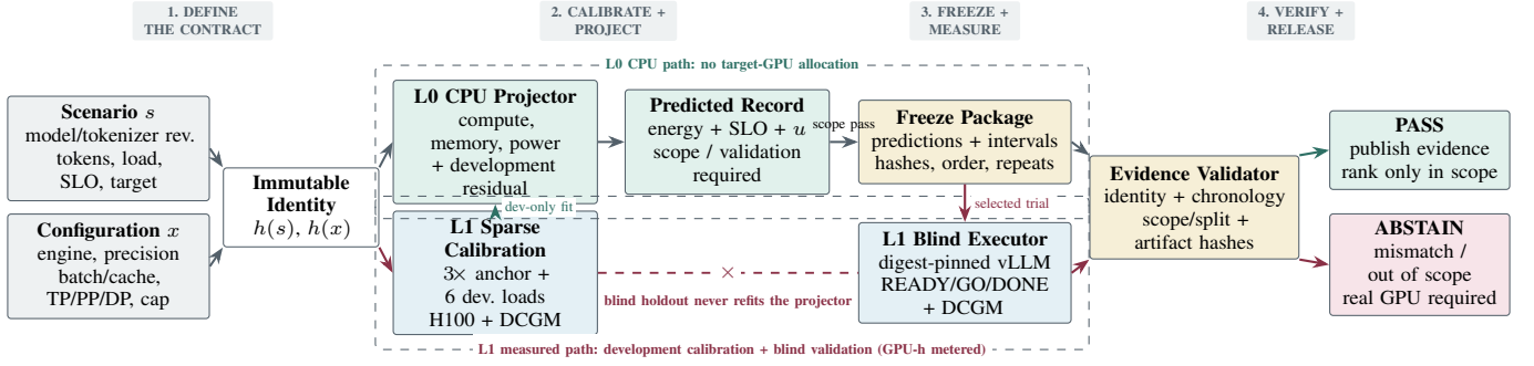
Fig. 1. End-to-end TokenPowerSandbox evidence flow. A workload scenario and serving configuration receive immutable identities before L0 screening or L1 execution. The CPU projector uses only development measurements for residual calibration; predictions, intervals, hashes, and run order are then frozen before selected blind H100 trials. The validator releases only identity-, chronology-, and scope-consistent evidence and otherwise abstains.
