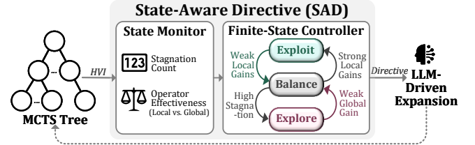
Figure 7: State-Aware Directive (SAD) workflow
