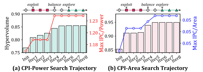
Figure 12: MCTS Search Progress over Iterations.
