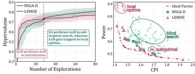
Figure 3: Left: Comparison of the LLM-driven and EA-based DSE methods. Right: Search results in the CPI–Power space.
