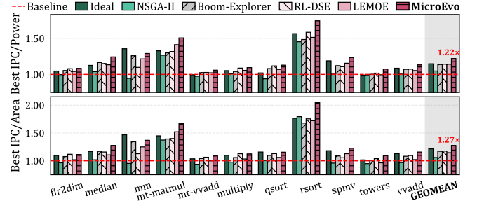
Figure 15: Relative IPC/Power and IPC/Area improvement over the RTL-aligned XiangShan Kunminghu baseline across benchmarks.
