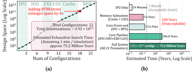
Figure 1: (a) The combinatorial explosion of the microarchitecture configurations. (b) Exhaustive search time for CPU design space.
