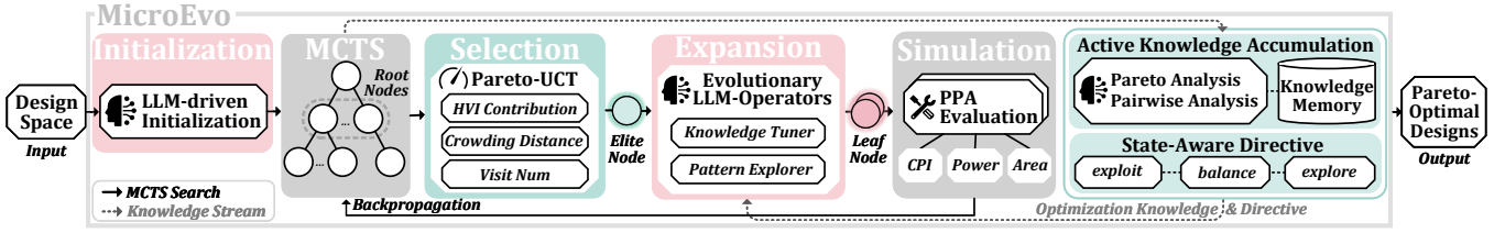
Figure 5: Overview of MicroEvo. LLM first initializes root designs, Pareto-UCT then selects elite nodes in the MCTS tree (Section 3.2), LLM-driven operators expand new nodes (Section 3.3), and PPA evaluation updates the tree, while active knowledge accumulation (Section 3.4) and state-aware directives (Section 3.5) continuously provide optimization guidance until the simulation budget is reached.
