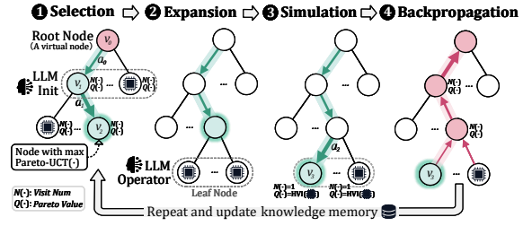
Figure 4: Evolutionary Monte Carlo Tree Search (MCTS) procedure.
