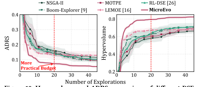
Figure 10: Hypervolume and ADRS comparison of different DSE methods versus number of explorations: the red dashed line marks a more practical evaluation budget of 20 trials.
