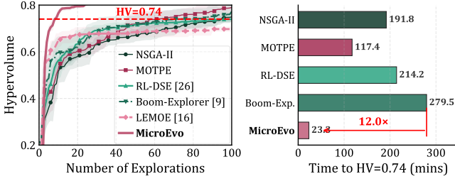
Figure 9: Convergence efficiency and time-to-target comparison.
