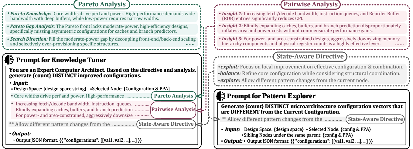
Figure 6: Prompt integration for LLM-driven expansion.
