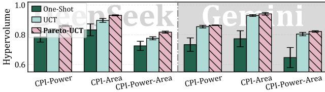
Figure 13: Effectiveness of the proposed Pareto-UCT.
