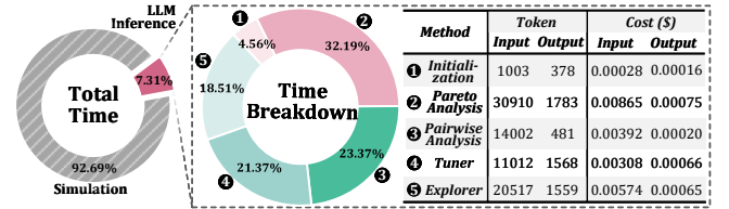
Figure 11: Token usage, cost, and total runtime breakdown of MicroEvo (DeepSeek-V3.2): 7.3% LLM inference vs. 92.7% simulation.
