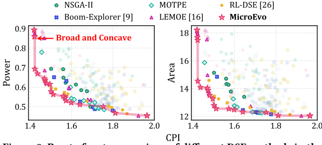
Figure 8: Pareto front comparison of different DSE methods in the CPI-Power and CPI-Area spaces.
