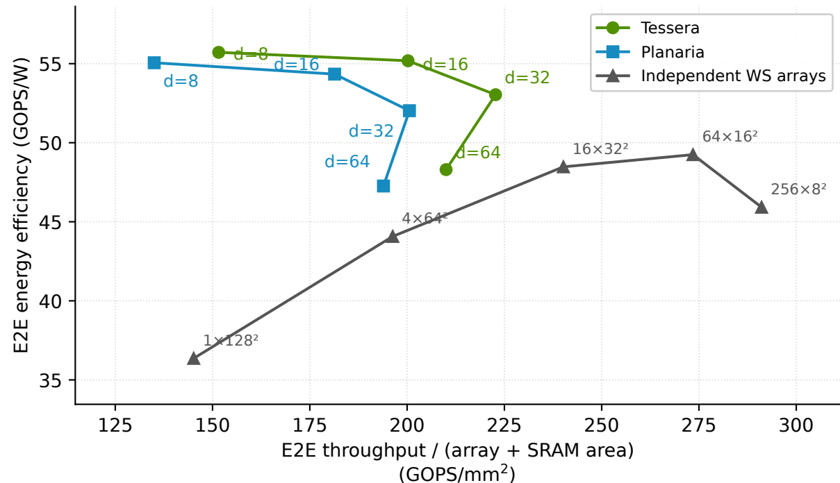
Joint EDP tiling · equal 128×128 PEs · HBM4 Geometric mean of 12 workloads
