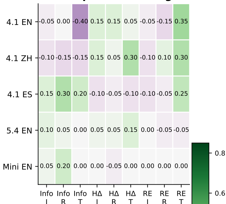
B Empirical coverage
