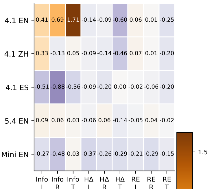
A Absolute mean deviation
