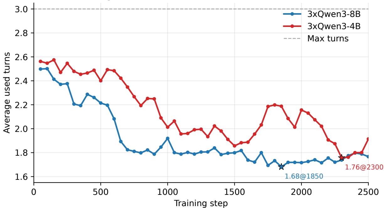
Average verification turns on held-out code tasks
