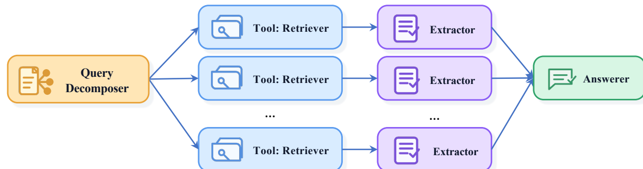
Workflow B · Retrieve–Extract–Answer (Search)
