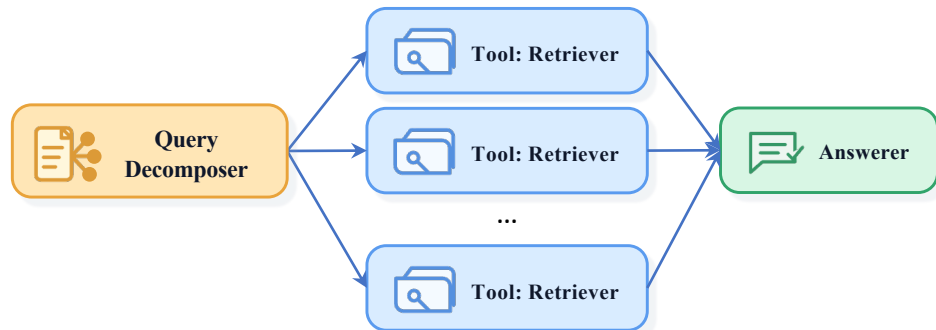
Workflow A · Parallel Retrieval (Search)
