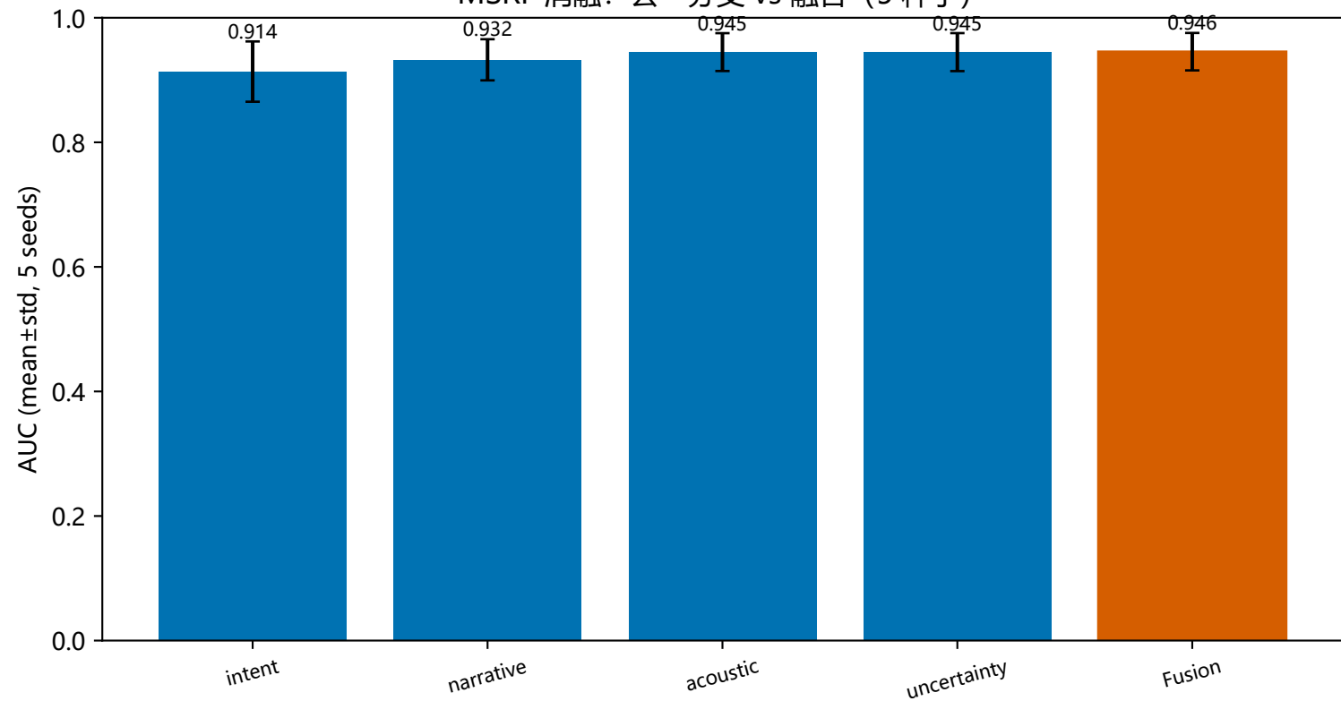
MSRF 消融：去一支 vs 融合 (5 种子)
