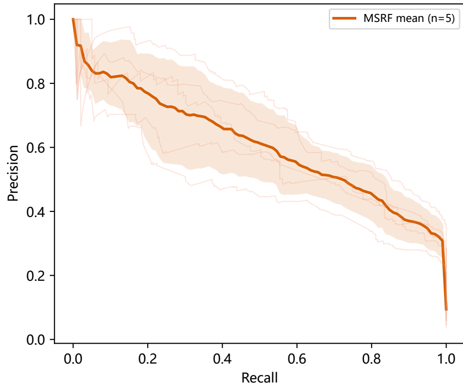
PR curve (real)
