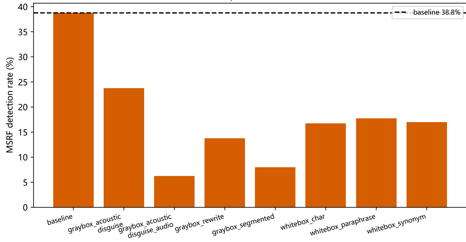
Detection rate under adaptive attacks (real fused detector)
