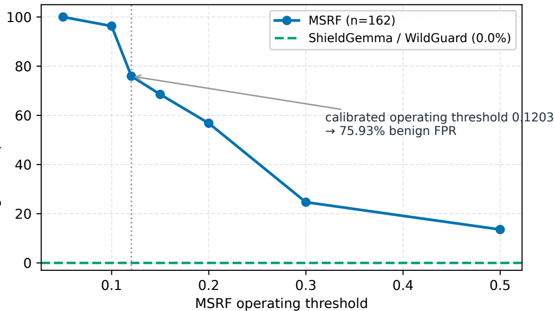
(a) Honest boundary: threshold does not transfer
