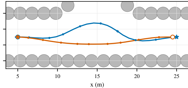
(b) TurboADMM-NL repair: validated
