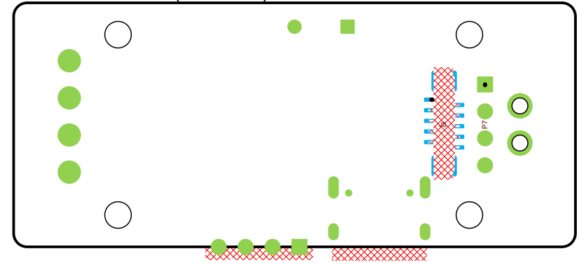
Bottom SMD/THT (Scale 2:1)
